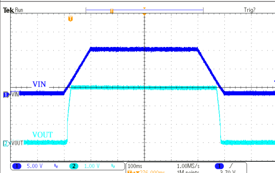
电源 ON/OFF 响应 HT73H30 ( V_{IN}=12V , I_{OUT}=180mA , T_{RISE}=T_{FALL}=100ms )
