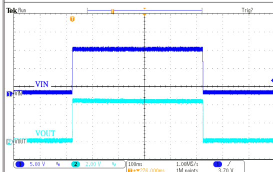
电源 ON/OFF 响应: HT73H44 ( V_{IN}=12V , I_{OUT}=250mA , T_{RISE}=T_{FALL}=0.1ms )
