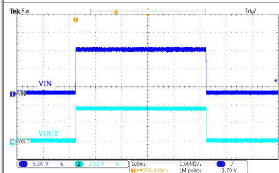
电源 ON/OFF 响应: HT73H36 ( V_{IN}=12V , I_{OUT}=250mA , T_{RISE}=T_{FALL}=0.1ms )
