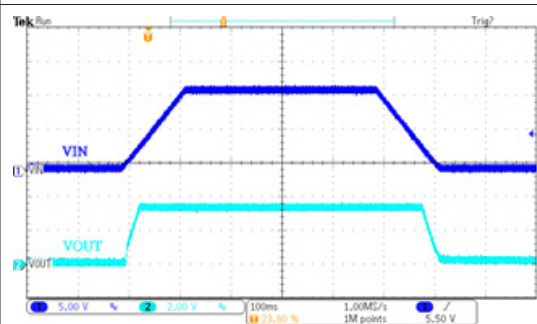
电源 ON/OFF 响应 HT73H33 ( V_{IN}=12V , I_{OUT}=250mA , T_{RISE}=T_{FALL}=100ms )
