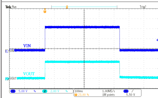
电源 ON/OFF 响应: HT73H33 ( V_{IN}=12V , I_{OUT}=0mA , T_{RISE}=T_{FALL}=0.1ms )
