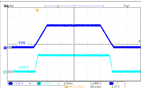
电源 ON/OFF 响应 HT73H36 ( V_{IN}=12V , I_{OUT}=250mA , T_{RISE}=T_{FALL}=100ms )
