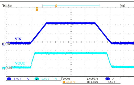
电源 ON/OFF 响应: HT73H33 ( V_{IN}=12V , I_{OUT}=0mA , T_{RISE}=T_{FALL}=100ms )
