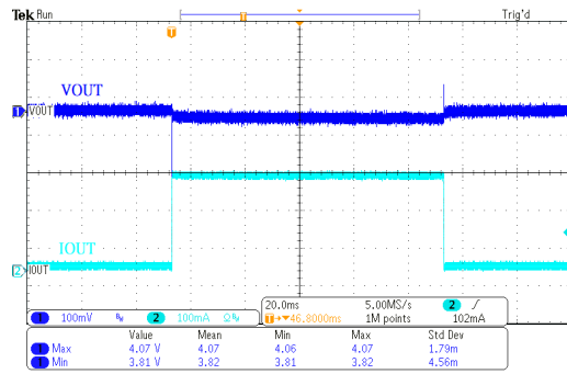
负载瞬态响应: HT73H40 ( V_{IN}=6V , I_{OUT}=10mA\sim 250mA )
