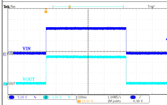
电源 ON/OFF 响应: HT73H50 ( V_{IN}=12V , I_{OUT}=250mA , T_{RISE}=T_{FALL}=0.1ms )
