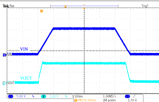
电源 ON/OFF 响应: HT73H36 ( V_{IN}=12V , I_{OUT}=0mA , T_{RISE}=T_{FALL}=100ms )
