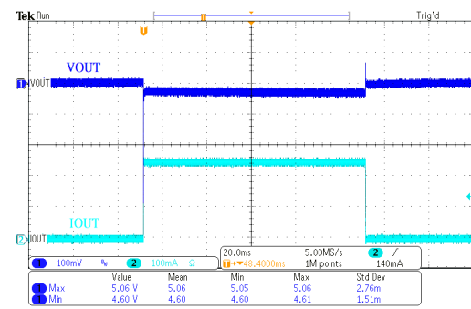
负载瞬态响应: HT73H50 ( V_{IN}=7V , I_{OUT}=0mA\sim 250mA )
