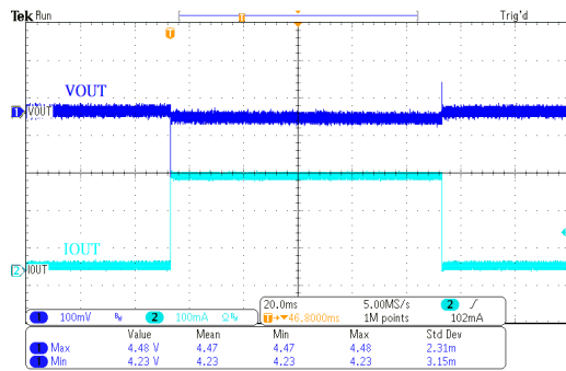
负载瞬态响应: HT73H44 ( V_{IN}=6.4V , I_{OUT}=10mA\sim 250mA )
