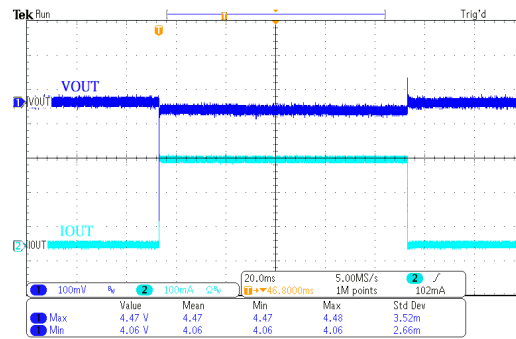
负载瞬态响应: HT73H44 ( V_{IN}=6.4V , I_{OUT}=0mA\sim 250mA )
