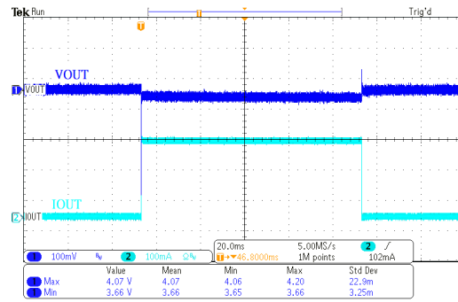
负载瞬态响应: HT73H40 ( V_{IN}=6V , I_{OUT}=0mA\sim 250mA )
