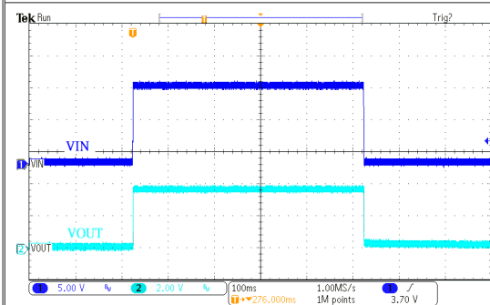
电源 ON/OFF 响应: HT73H36 ( V_{IN}=12V , I_{OUT}=0mA , T_{RISE}=T_{FALL}=0.1ms )
