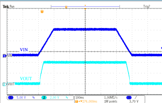
电源 ON/OFF 响应 HT73H40 ( V_{IN}=12V , I_{OUT}=250mA , T_{RISE}=T_{FALL}=100ms )
