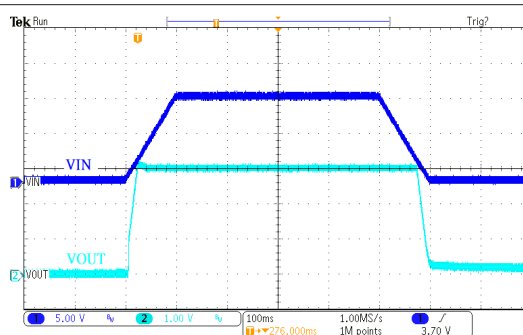
电源 ON/OFF 响应: HT73H30 ( V_{IN}=12V , I_{OUT}=0mA , T_{RISE}=T_{FALL}=100ms )
