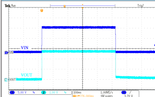
电源 ON/OFF 响应: HT73H27 ( V_{IN}=12V , I_{OUT}=0mA , T_{RISE}=T_{FALL}=0.1ms )
