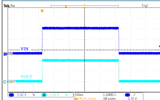
电源 ON/OFF 响应: HT73H40 ( V_{IN}=12V , I_{OUT}=250mA , T_{RISE}=T_{FALL}=0.1ms )
