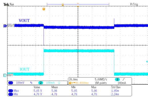
负载瞬态响应: HT73H50 ( V_{IN}=7V , I_{OUT}=10mA\sim 250mA )
