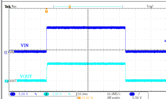
电源 ON/OFF 响应: HT73H33 ( V_{IN}=12V , I_{OUT}=250mA , T_{RISE}=T_{FALL}=0.1ms )
