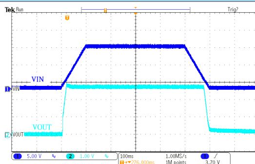
电源 ON/OFF 响应: HT73H27 ( V_{IN}=12V , I_{OUT}=0mA , T_{RISE}=T_{FALL}=100ms )
