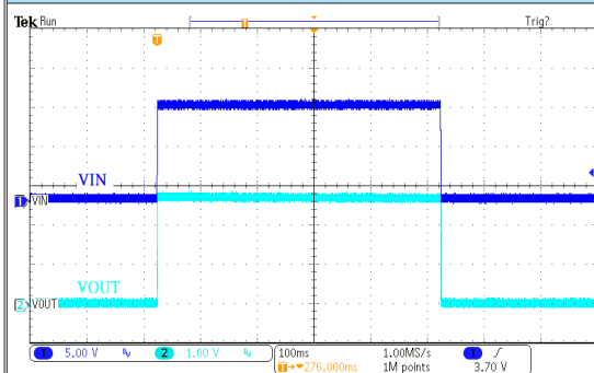
电源 ON/OFF 响应 HT73H27 ( V_{IN}=12V , I_{OUT}=180mA , T_{RISE}=T_{FALL}=0.1ms )
