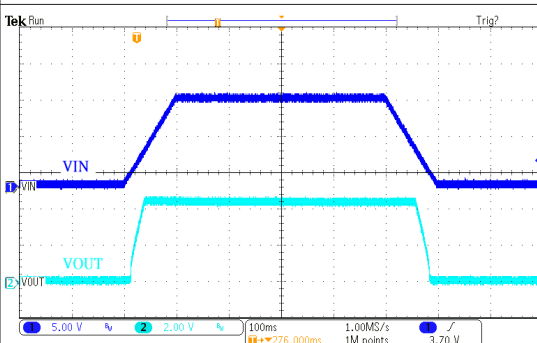
电源 ON/OFF 响应 HT73H44 ( V_{IN}=12V , I_{OUT}=250mA , T_{RISE}=T_{FALL}=100ms )
