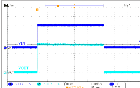
电源 ON/OFF 响应 HT73H30 ( V_{IN}=12V , I_{OUT}=180mA , T_{RISE}=T_{FALL}=0.1ms )
