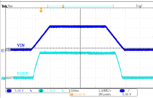
电源 ON/OFF 响应: HT73H50 ( V_{IN}=12V , I_{OUT}=250mA , T_{RISE}=T_{FALL}=100ms )
