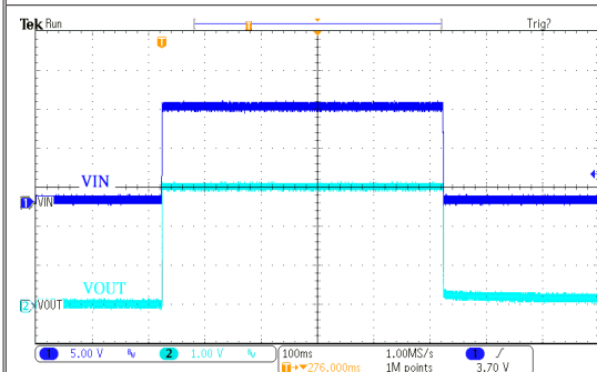
电源 ON/OFF 响应: HT73H30 ( V_{IN}=12V , I_{OUT}=0mA , T_{RISE}=T_{FALL}=0.1ms )
