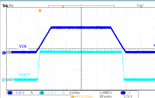
电源 ON/OFF 响应 HT73H27 ( V_{IN}=12V , I_{OUT}=180mA , T_{RISE}=T_{FALL}=100ms )
