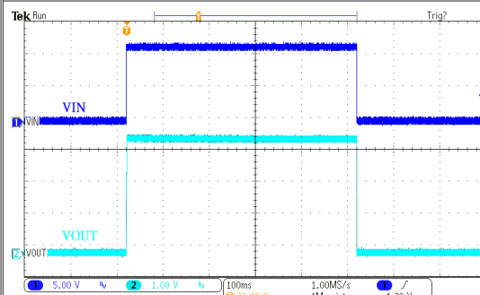
电源 ON/OFF 响应: HT75H36
