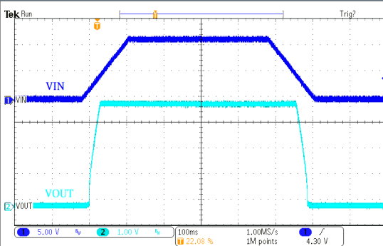
电源 ON/OFF 响应 HT75H40 ( V_{IN}=12V , I_{OUT}=150mA , T_{RISE}=T_{FALL}=100ms )
