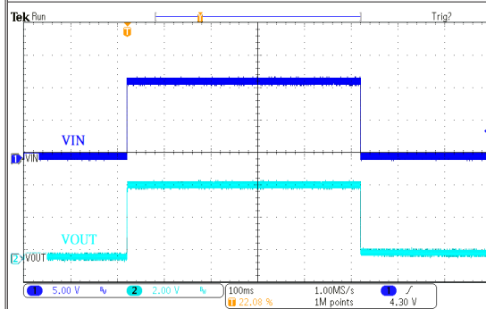
电源 ON/OFF 响应: HT75H44 ( V_{IN}=12V , I_{OUT}=0mA , T_{RISE}=T_{FALL}=0.1ms )
