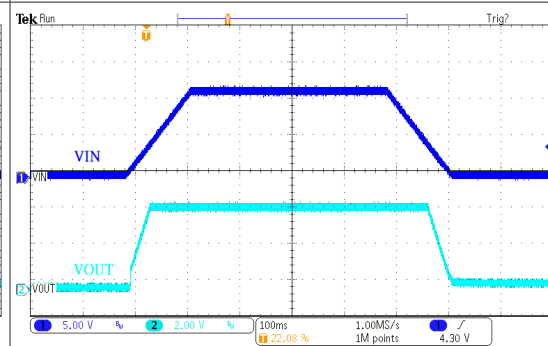
电源 ON/OFF 响应: HT75H44 ( V_{IN}=12V , I_{OUT}=0mA , T_{RISE}=T_{FALL}=100ms )
