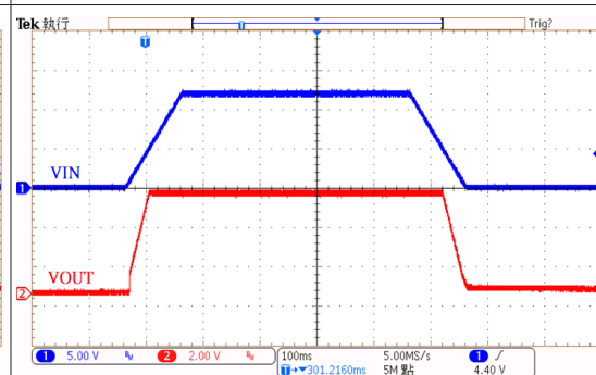
电源 ON/OFF 响应: HT75H50 ( V_{IN}=12V , I_{OUT}=0mA , T_{RISE}=T_{FALL}=100ms )
