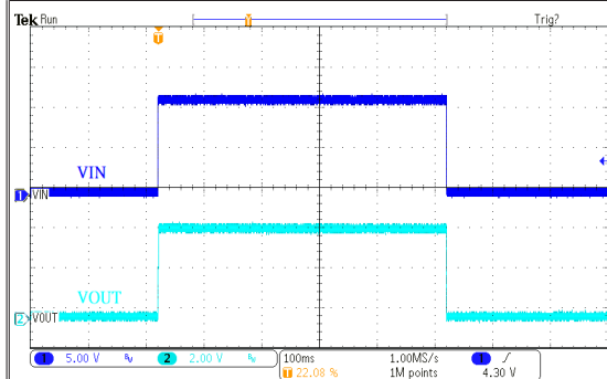
电源 ON/OFF 响应: HT75H44 ( V_{IN}=12V , I_{OUT}=150mA , T_{RISE}=T_{FALL}=0.1ms )
