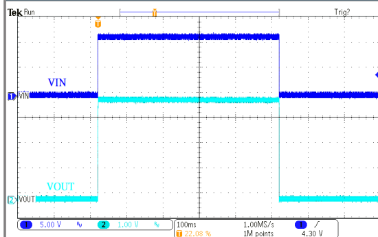
电源 ON/OFF 响应: HT75H40 ( V_{IN}=12V , I_{OUT}=150mA , T_{RISE}=T_{FALL}=0.1ms )
