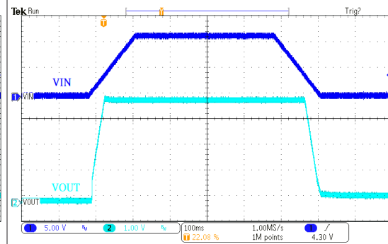
电源 ON/OFF 响应: HT75H40 ( V_{IN}=12V , I_{OUT}=0mA , T_{RISE}=T_{FALL}=100ms )
