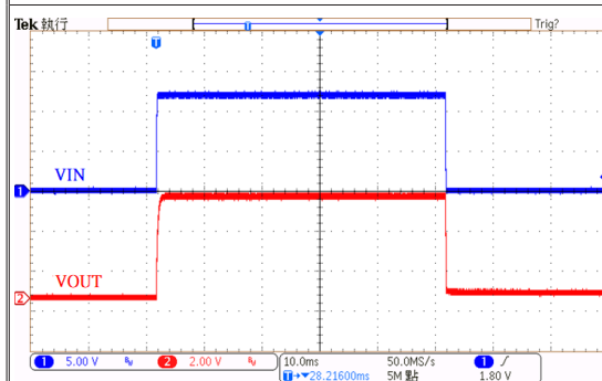
电源 ON/OFF 响应: HT75H50 ( V_{IN}=12V , I_{OUT}=0mA , T_{RISE}=T_{FALL}=0.1ms )
