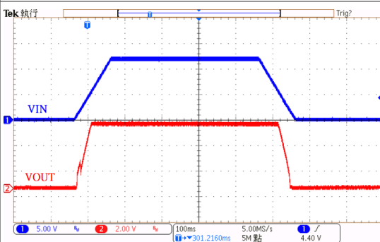
电源 ON/OFF 响应: HT75H50 ( V_{IN}=12V , I_{OUT}=150mA , T_{RISE}=T_{FALL}=100ms )
