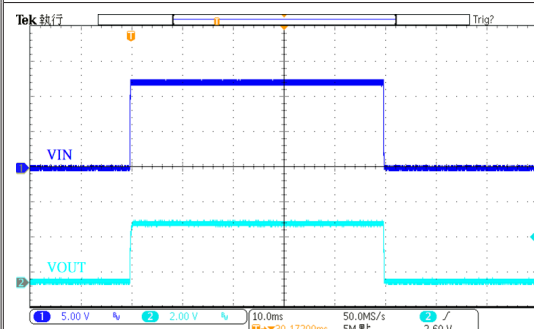
电源 ON/OFF 响应: HT75H33
