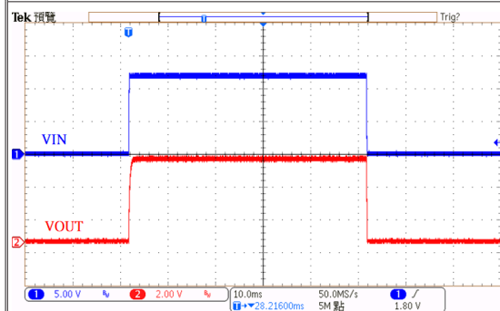
电源 ON/OFF 响应: HT75H50 ( V_{IN}=12V , I_{OUT}=150mA , T_{RISE}=T_{FALL}=0.1ms )
