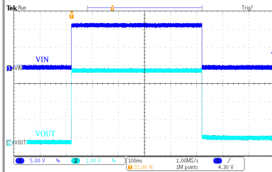
电源 ON/OFF 响应: HT75H40 ( V_{IN}=12V , I_{OUT}=0mA , T_{RISE}=T_{FALL}=0.1ms )
