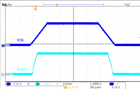
电源 ON/OFF 响应 HT75H44 ( V_{IN}=12V , I_{OUT}=150mA , T_{RISE}=T_{FALL}=100ms )
