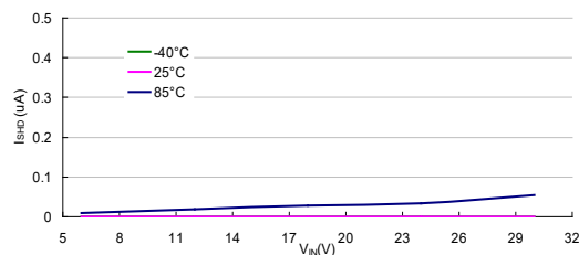
I_{SHD} vs V_{IN} : HT7533-7 ( I_{OUT}=0mA )
