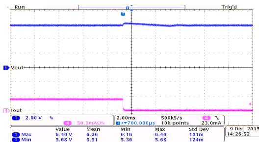
负载瞬态响应: HT7560-7 ( V_{IN}=8.0V , I_{OUT}=40mA to 0mA )
