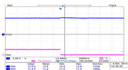
负载瞬态响应: HT75C0-7 ( V_{IN}=14V , I_{OUT}=40mA to 0mA )
