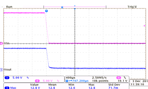
掉电响应: HT75C0-7 ( I_{OUT}=0mA , T_{FALL}=0.1ms )
