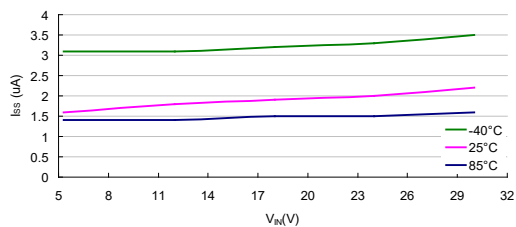
I_{SS} vs V_{IN} : HT7533-7 ( I_{OUT}=0mA )
