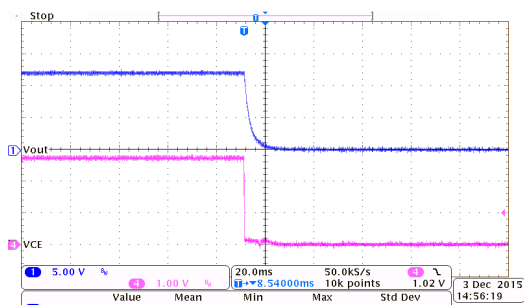
开关响应: HT75C0-7 ( I_{OUT}=150mA , V_{CE}=2.7V to 0V)
