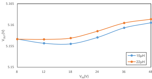
线性调整率 (HT7463C, V OUT =5V, I OUT =300mA)
