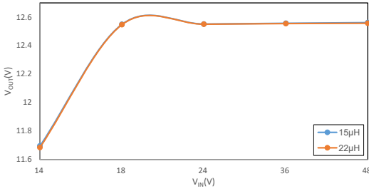
线性调整率 (HT7463C, V OUT =12.5V, I OUT =300mA)
