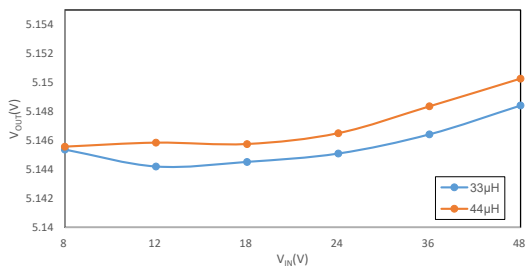
线性调整率 (HT7463D, V OUT =5V, I OUT =300mA)
