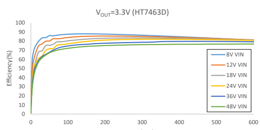
效率 vs. 负载 (HT7463D, V_{OUT}=3.3V )
