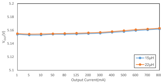
负载调整率 (HT7463C, V_{OUT}=5V )
