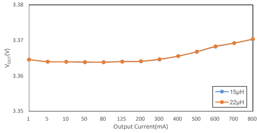
负载调整率 (HT7463C, V OUT =3.3V)
