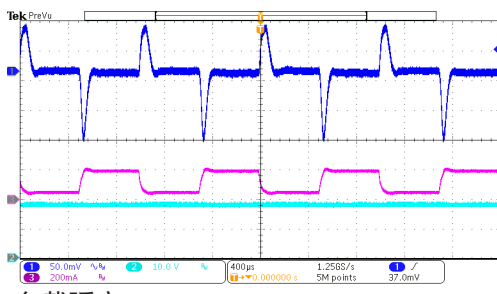
负载瞬变 (HT7463C, I OUT =50mA~200mA)
