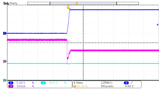
短路恢复 (HT7463C, I_{OUT}=500mA )
