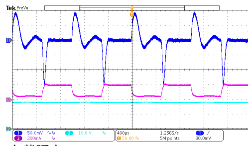
负载瞬变 (HT7463D, I OUT =50mA~200mA)
