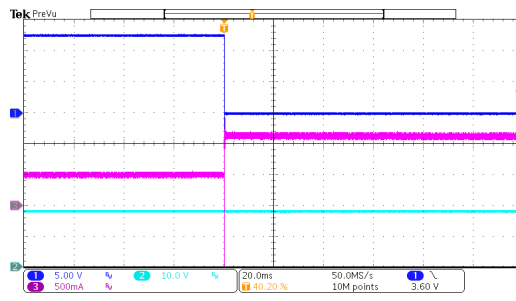
输出短路 (HT7463D, I_{OUT}=500mA )
