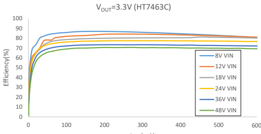
效率 vs. 负载 (HT7463C, V_{OUT}=3.3V )
