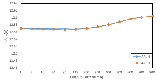
负载调整率 (HT7463D, V_{OUT}=12.5V )
