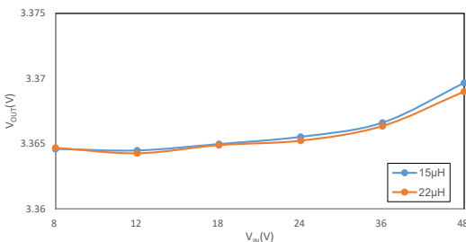
线性调整率 (HT7463C, V OUT =3.3V, I OUT =300mA)
