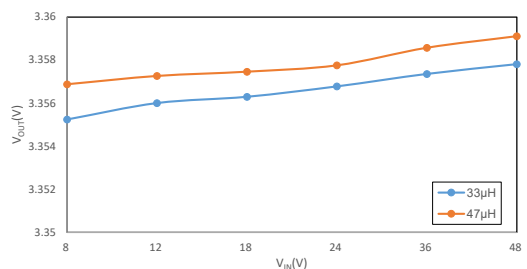
线性调整率 (HT7463D, V OUT =3.3V, I OUT =300mA)
