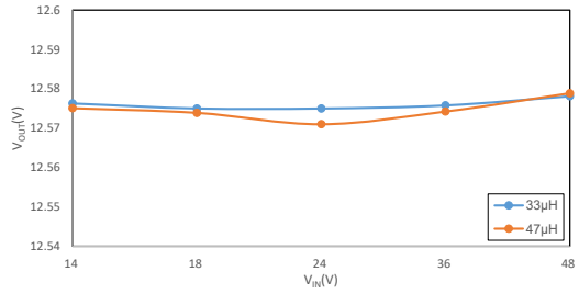
线性调整率 (HT7463D, V OUT =12.5V, I OUT =300mA)
